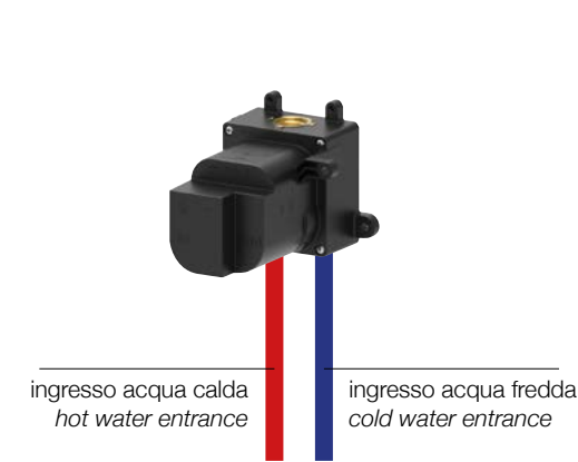
MODULO INCASSO TERMOSTATICO THERMOSTAT CONCEALED MODULE
