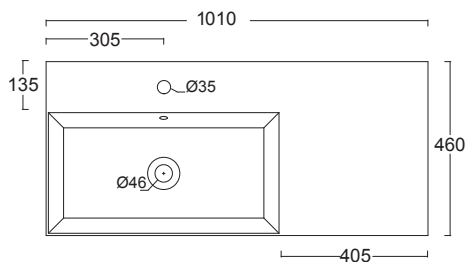
34360101 Lavabo SPY 101x46 Plan 34360101 Washbasin SPY 101x46 Plan
