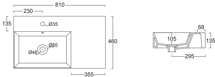
34340101 Lavabo SPY 81x46 Plan 34340101 Washbasin SPY 81x46 Plan
