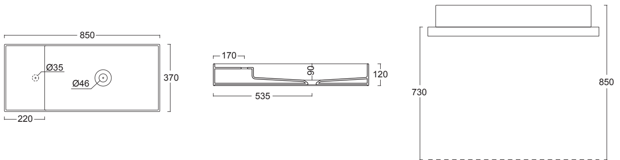
31100101 Lavabo HIDE 85x37 31100101 Washbasin HIDE 85x37
